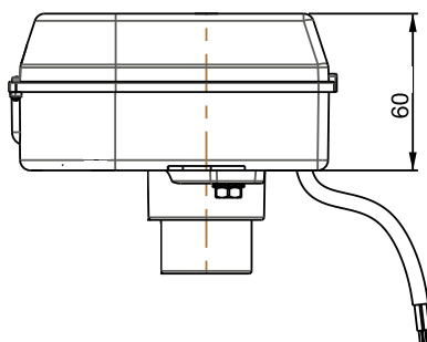
Actuator with Clip system- 4930 / 4950
