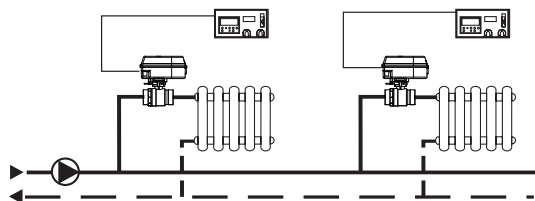
Actuator 4230 with FBV 600 valve installation example
