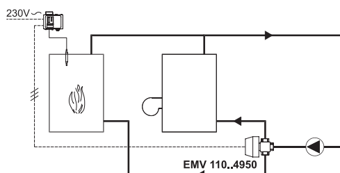
Actuator 4950 with FBV 230C-L valve installation example
