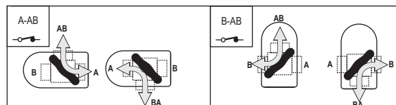
A-AB and B-AB installation layout.
