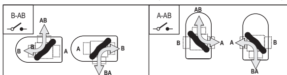
B-AB and A-AB installation layout.
