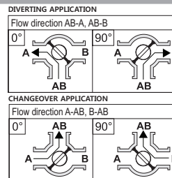
A-AB and B-AB installation layout.
