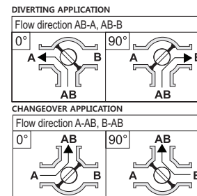
A-AB and B-AB installation layout.
